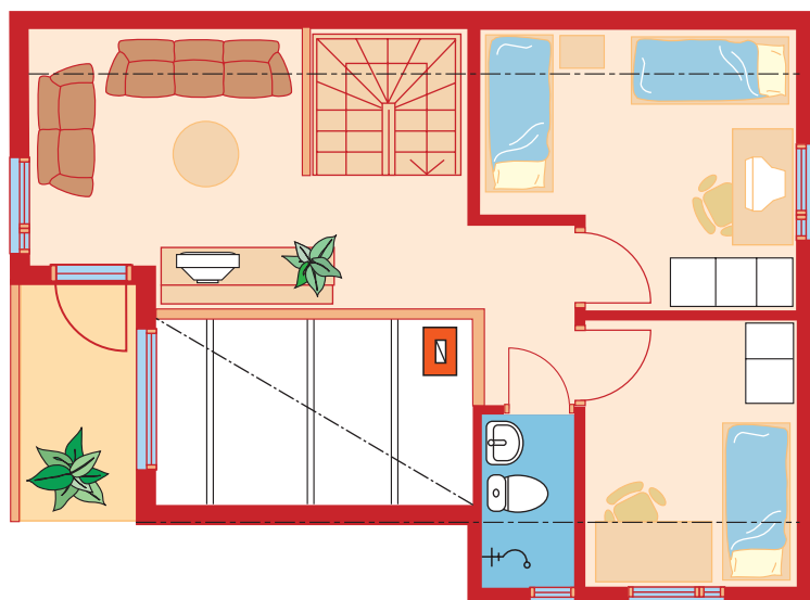
Upstairs 1:100
