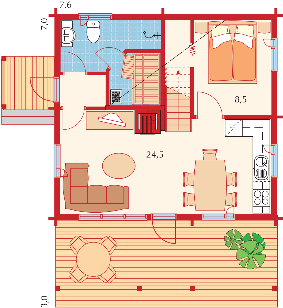
Downstairs 1:75
