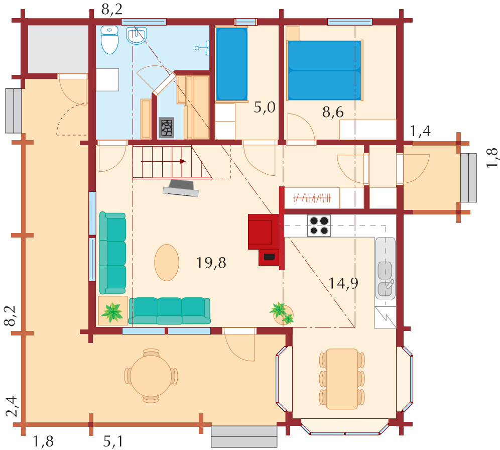
Downstairs 1:100
